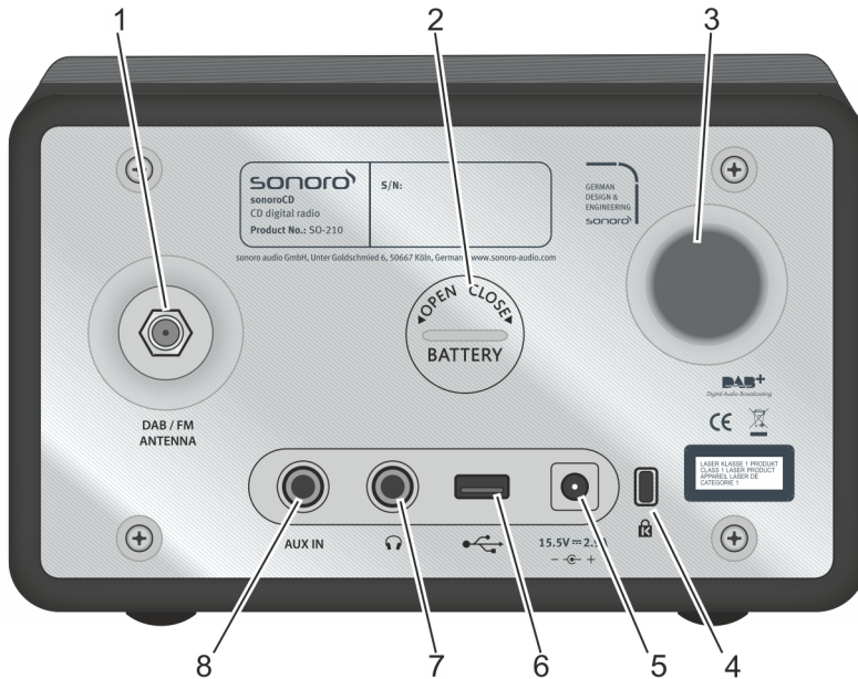
Fig. 3: sonoroCD rear view
